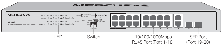
Figure 1-4 Front Panel of MS120GP
